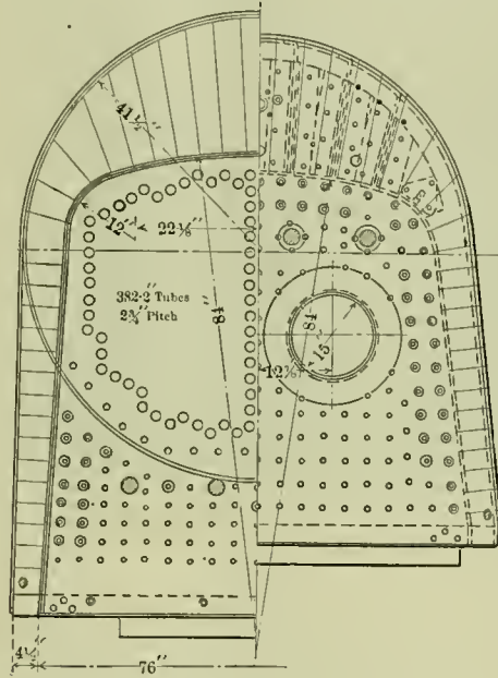
SECTION AND ELEVATION OF FIREBOX.
